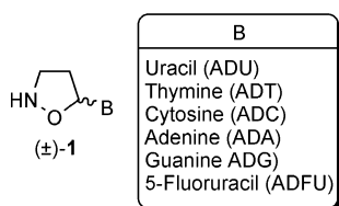
Figure 1. Isoxazolidinyl nucleosides.
